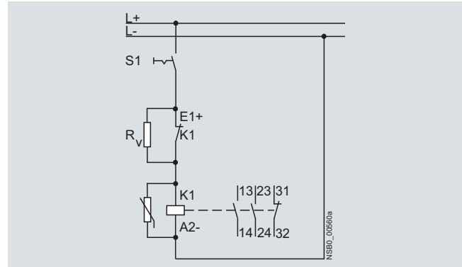
Circuit diagram
