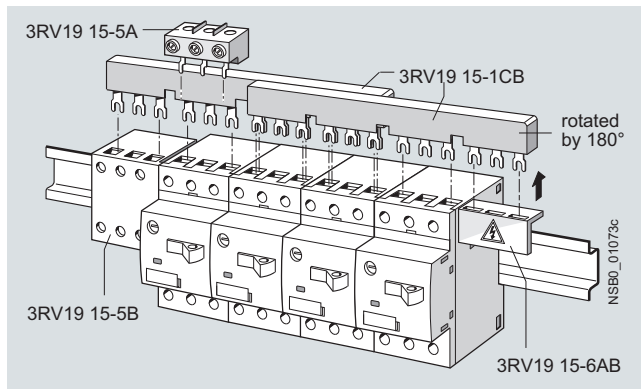
3-phase busbar system SIRIUS, size S00
